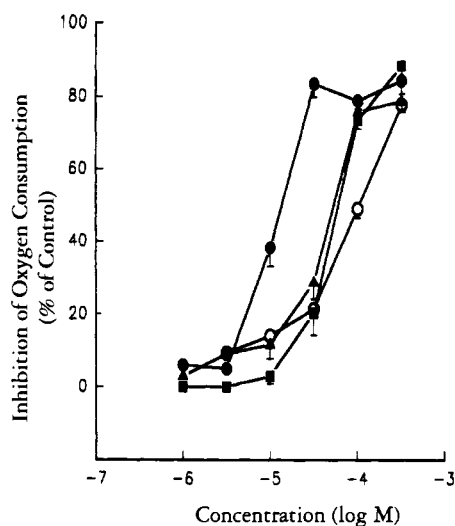
FIGURE 1. Concentration-response curves for emodin [2] (●), alizarin [13] (■), alizarin complexone [14] (▲), and α-tocopherol (○) in inhibiting FeSO 4 -induced oxygen consumption in rat heart mitochondria. Each data point is the mean ± s.e.m. for three different samples.
