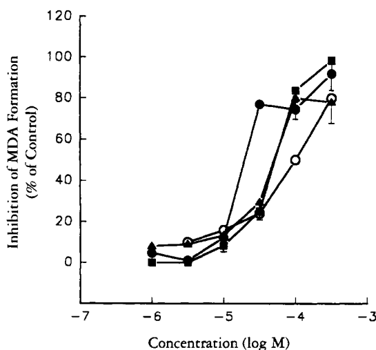
FIGURE 2. Concentration-response curves for emodin [2] (●), alizarin [13] (■), alizarin complexone [14] (▲), and α-tocopherol (○) in inhibiting FeSO 4 -induced MDA formation in rat heart mitochondria. Each data point is the mean ± s.e.m. for three different samples.
